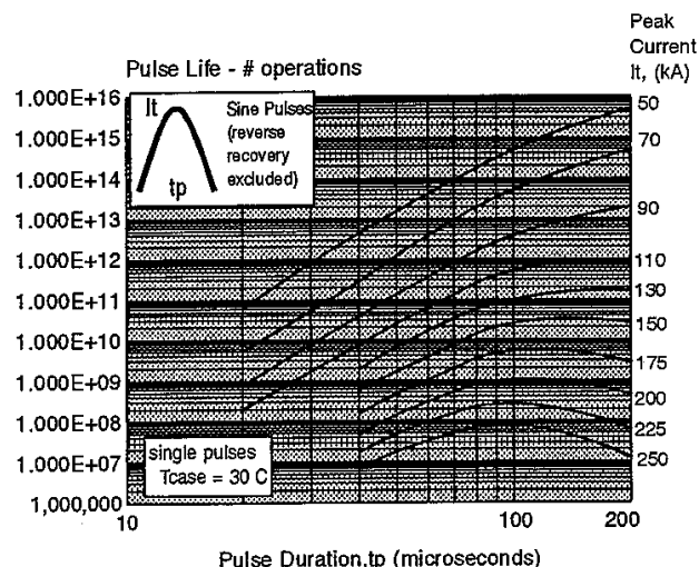
FIGURE 3. SINUSOIDAL, SINGLE SHOT CAPABILITY
