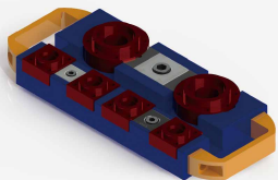
▲ 快速換模加工治具範例 Single-minute exchange of die(SMED) processing jig
