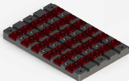
▲ 油壓缸蓋超量產治具範例 Hydraulic cylinder cover processing jig
