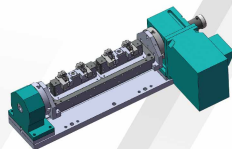
四軸治具(可加工3面) Jigs on the 4th axis (Available for machining 3 side)
