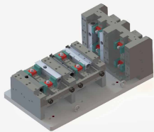
▲ 關門器加工治具範例 Door closer processing jig
