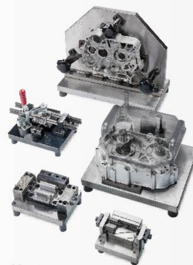
檢具 ▲ Custom inspection device
