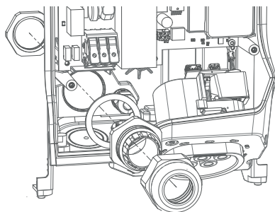
Rear gland assembly
