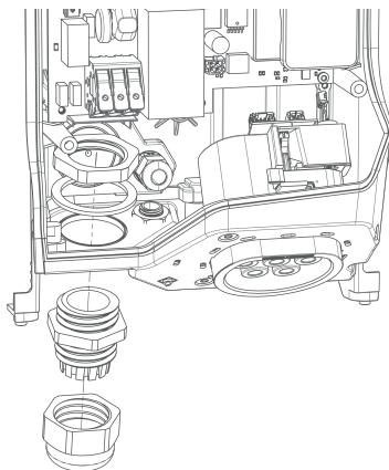
Bottom gland assembly
