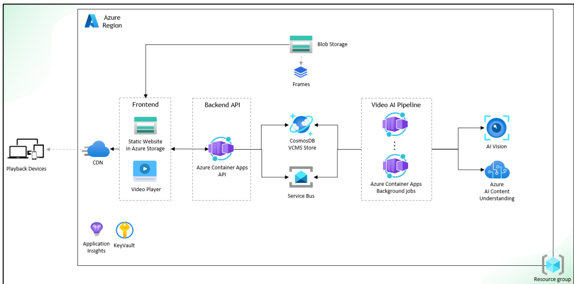
Smart Cropping solution architecture diagram
