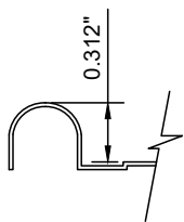
COVE JOINT
