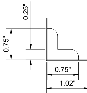
2 VersaLiner™ END VIEW
