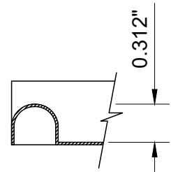
COVE JOINT
