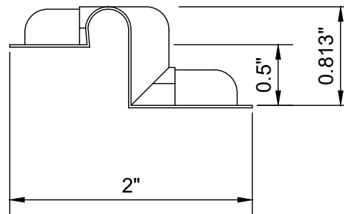
2 VersaLiner™ END VIEW
