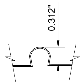
COMPRESSION JOINT (TYP.) A
