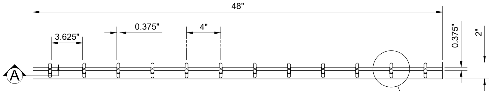
1 VersaLiner™ TOP VIEW
