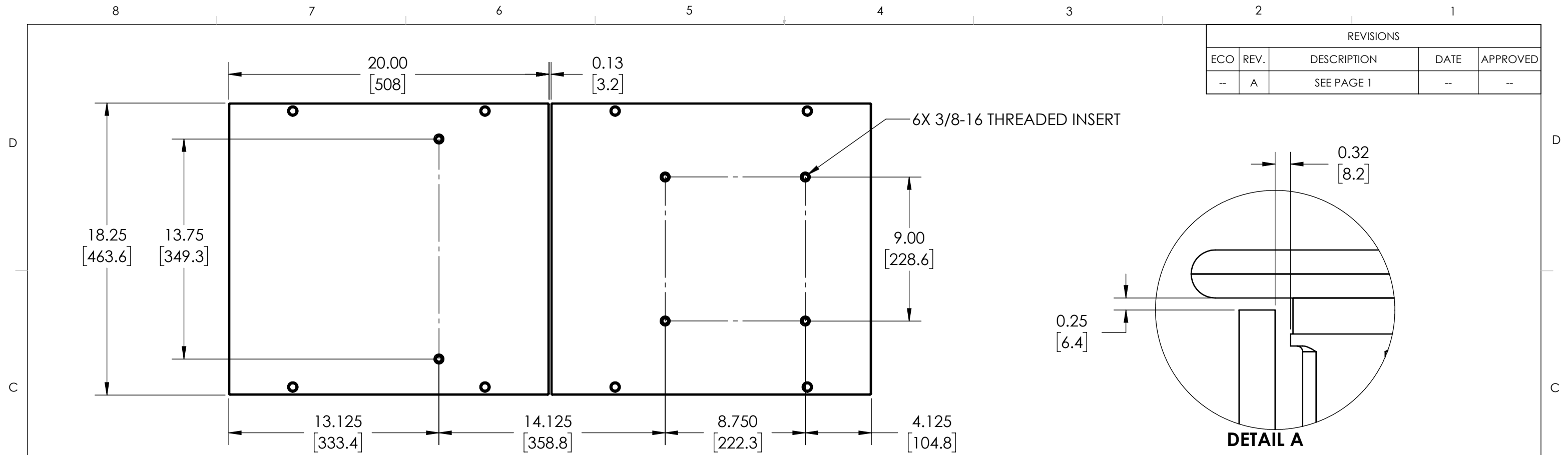
TOP OF PLATES (STAIRS REMOVED)
