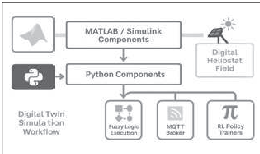
Fig. 3: Digital twin workflow integrating sensor simulators, fuzzy logic execution engine, MQTT broker, and RL policy trainers
