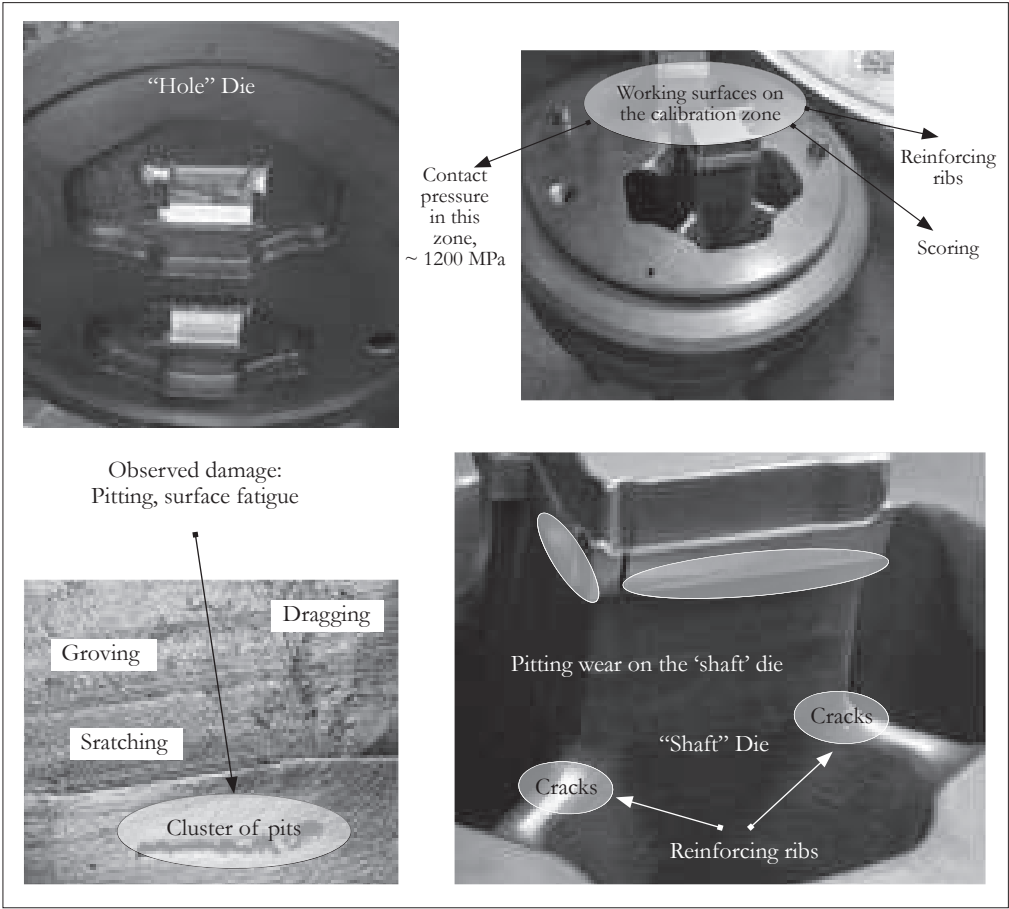
Figure 1. Typical localization of defects on the working surfaces and reinforcing ribs of the extrusion die. The two upper images show, respectively, the hollow die (hole die) and the shaft die. The two lower images show the corresponding defects or damage observed on the working surfaces and reinforcing ribs of these dies. Source: Everest sh.a. (2025).
