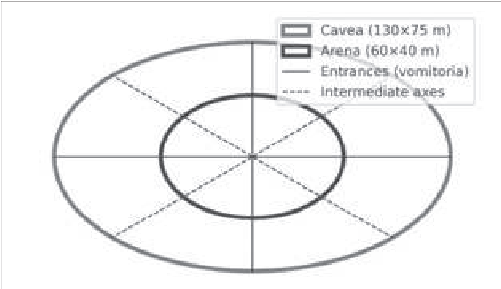
Fig 4. Approximate dimensions of the amphitheatre ( 130 \times 75 m).
