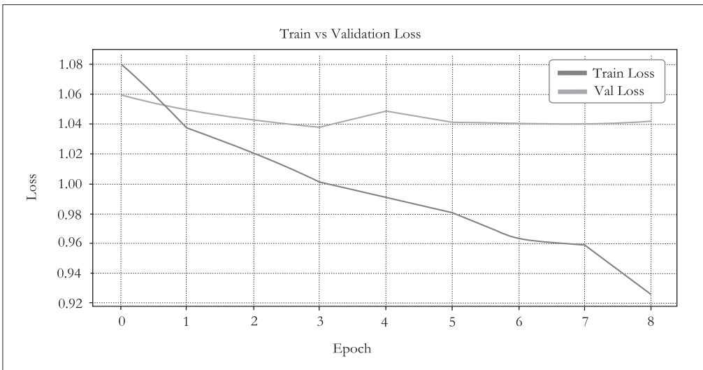
Figure 13. Train vs validation loss curve-BiLSTM+Attention+MFCC
