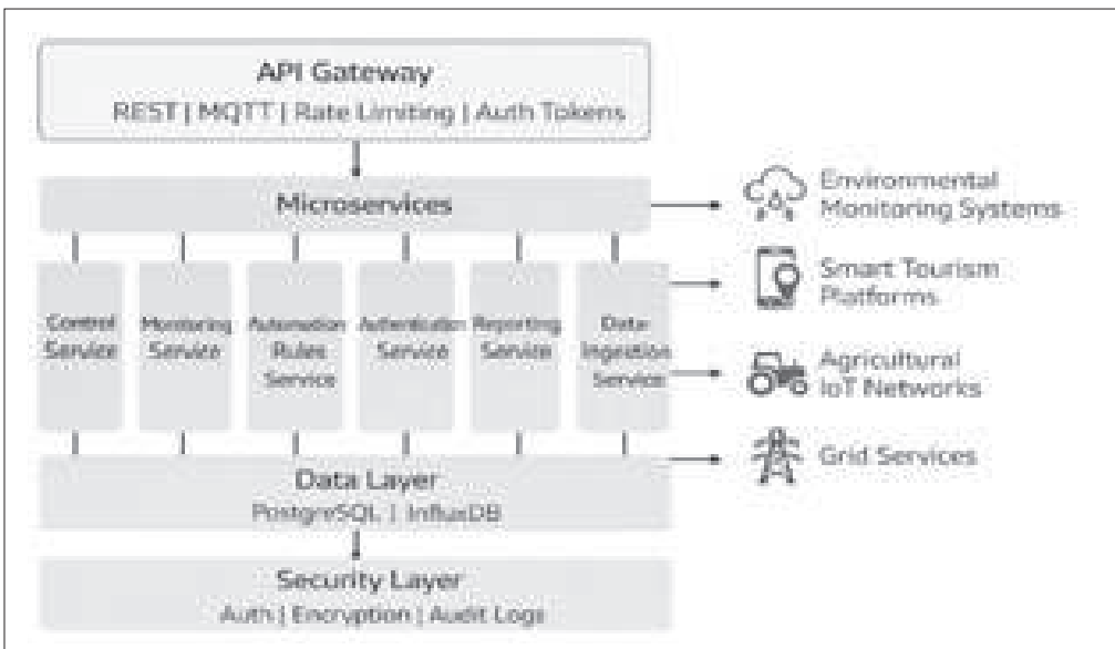
Fig. 6: Microservices and API gateway structure enabling secure, scalable, and interoperable platform-level integration
