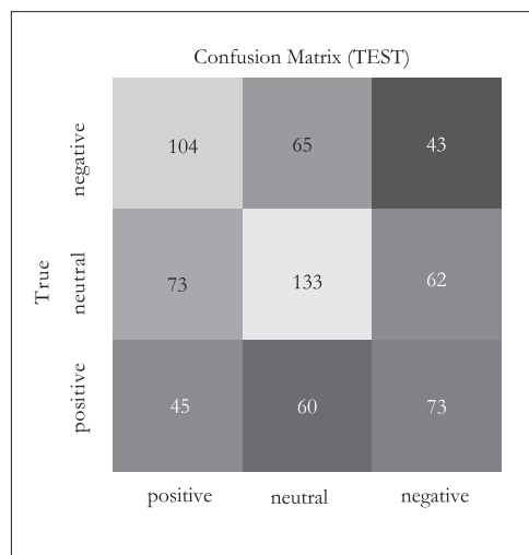
Figure 15. Confusion matrix for BiLSTM with Attention after class weight loss
