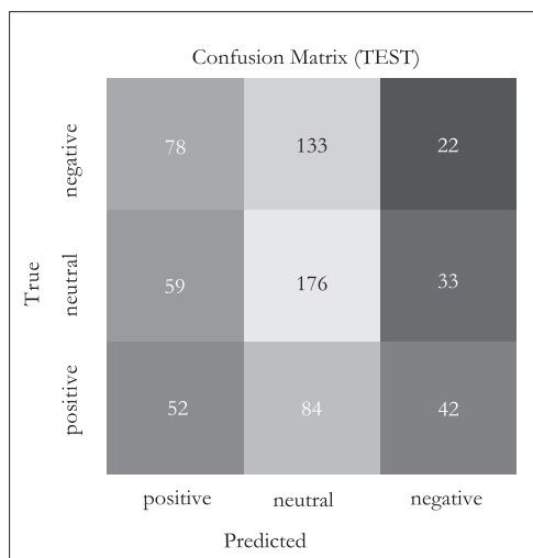
Figure 14. Confusion matrix for BiLSTM with Attention before class weight loss
