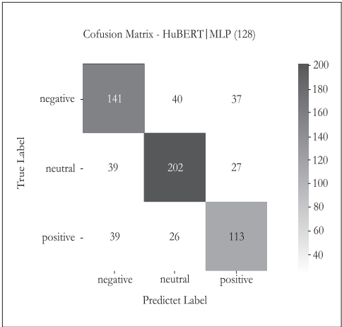
Figure 10. Confusion Matrix for HuBERT for MLP Classifier
