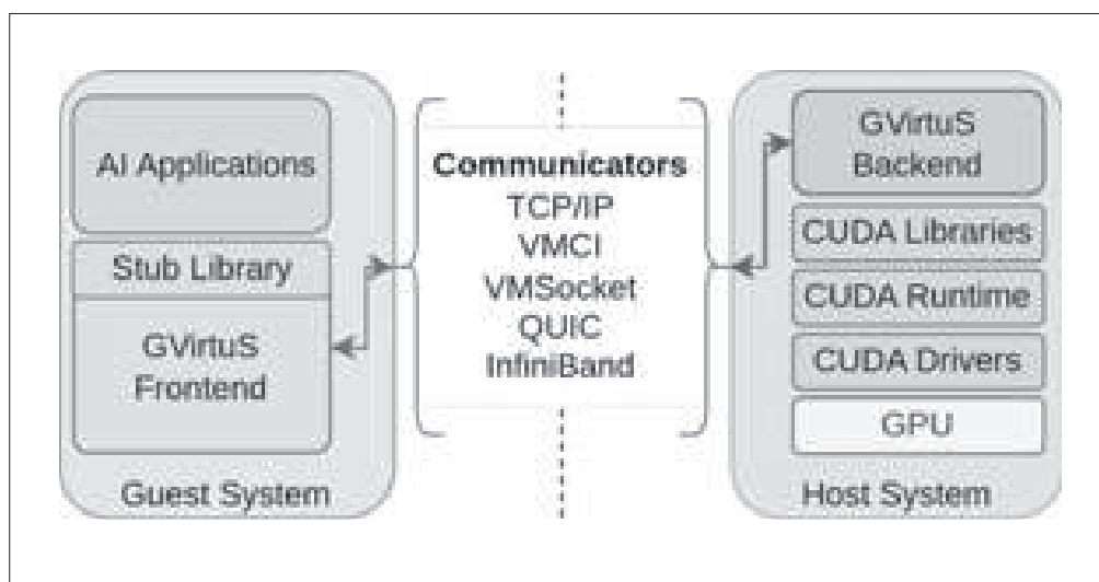
Figure 2. Overview of the GVirtuS components and system architecture.
