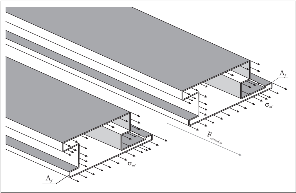
Figure 2. Schematic of the extrusion configuration showing the billet and resulting dual profiles, with annotated vectors of extrusion force ( F ), corrected flow stress, \sigma'_m .
