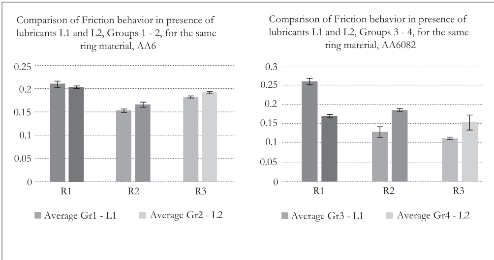
Figure 15. Comparison of lubricants L1 and L2 for AA6063 and AA6082 alloys, respectively Groups 1-2 and 3-4. Lower \mu indicates better lubrication performance.
