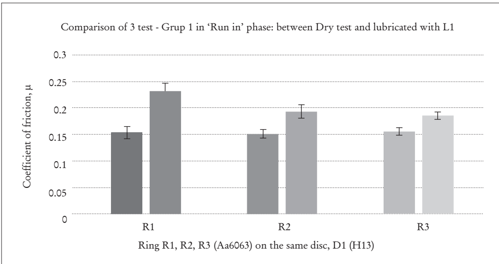
Figure 7. Comparison of the performance of three AA6063 rings sliding against the H13 disc under dry and L1-lubricated run-in conditions.
