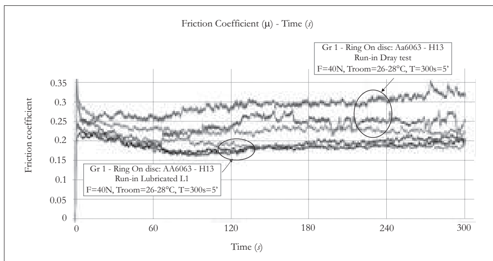
Figure 6. Comparison of friction coefficient ( \mu ) during the ‘run-in’ phase in Group 1 under dry contact and lubricated conditions with L1. Ring – AA6063 on Disc – H13 surrogate
