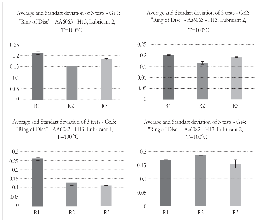
Figure 14. Average friction coefficient and standard deviation for each test group during main test phase - steady state, from 15' to 20' (Microsoft Corporation, 2025)
