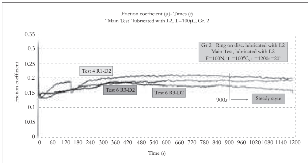
Figure 11. Friction coefficient over time during main test (1200 sec) with lubricant L2. Steady-state region indicated after 900 sec – for Group 2.
