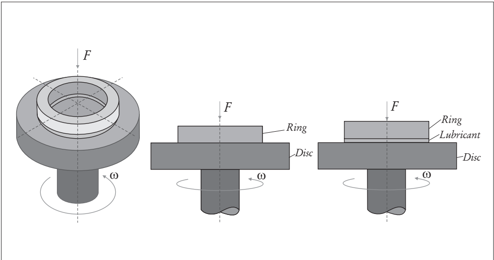
Figure 5. Schematic representation of ring on disc contact, without (dry test) and with lubricant
