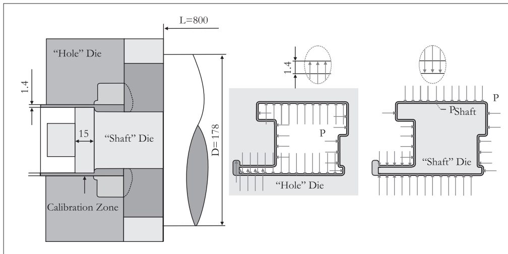
Figure 3. Schematic representation of contact pressure distribution on the calibration surfaces of the die pair
