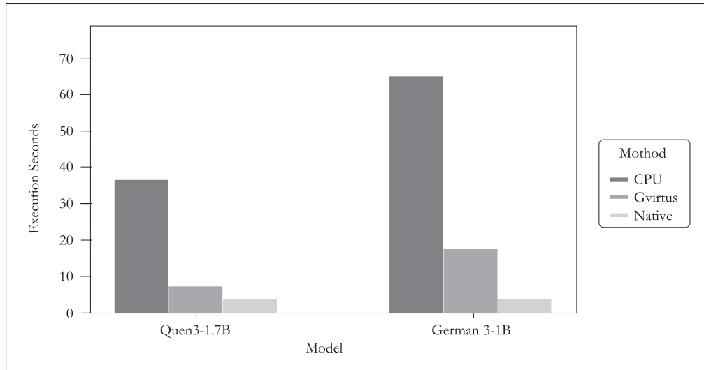
Figure 3. LLMs test. Performance comparison of two LLMs across three different hardware setups after 100 execution runs. The mean execution time and standard deviation for Quen3-1.7B are 36.25 \pm 5.16 seconds on the CPU-only setup, 7.01 \pm 0.86 seconds using GVirtuS, and 3.20 \pm 0.41 seconds on the native GPU. For Gemma3-1B, the CPU-only execution requires 64.66 \pm 10.58 seconds; GVirtuS takes 17.25 \pm 2.44 seconds, and the native GPU completes the task in 2.54 \pm 0.96 seconds.
