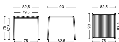
PALISSADE TABLE Length 82,5 cm Width 90 cm Height 75 cm Weight 17,9 kg
