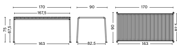
PALISSADE TABLE Length 170 cm Width 90 cm Height 75 cm Weight 31,55 kg
