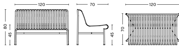
PALISSADE DINING BENCH W/O ARMREST Width 120 cm Depth 70 cm Height 80 cm Seat height 45 cm Weight 19 kg
