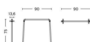
PALISSADE MIDDLE LEG Width 90 cm Depth 13,6 cm Height 75 cm Weight 3,48 kg
