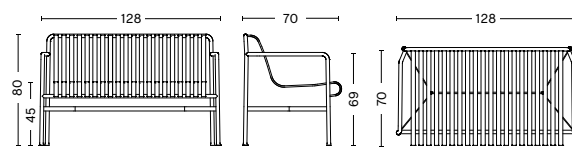
PALISSADE DINING BENCH Width 128 cm Depth 70 cm Height 80 cm Seat height 45 cm Weight 20 kg
