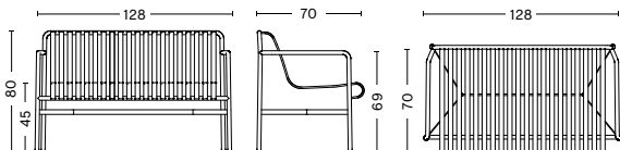
PALISSADE DINING BENCH Width 128 cm Depth 70 cm Height 80 cm Seat height 45 cm Weight 20 kg
