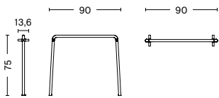
PALISSADE MIDDLE LEG Width 90 cm Depth 13,5 cm Height 75 cm Weight 3,48 kg
