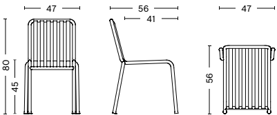
PALISSADE CHAIR Width 47 cm Depth 56 cm Height 80 cm Seat height 45 cm Seat depth 41 cm Weight 7,93 kg
