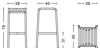
PALISSADE BAR STOOL Width 38 cm Depth 45 cm Height 78 cm Weight 8 kg
