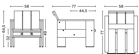
CRATE LOUNGE CHAIR Width 58 cm Depth 77 cm Height 64,5 cm Seat height 32 cm Seat depth 44,5 cm
