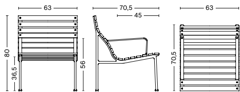
TRAVERSE LOUNGE ARMCHAIR Width 63 cm Depth 70,5 cm Height 80 cm Seat height 36,5 cm Seat depth 45 cm
