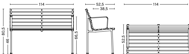
TRAVERSE DINING BENCH W ARMREST Width 114 cm Depth 52,5 cm Height 80,5 cm Seat height 46 cm Seat depth 38,5 cm
