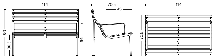
TRAVERSE LOUNGE BENCH W ARMREST Width 114 cm Depth 70,5 cm Height 80 cm Seat height 36,5 cm Seat depth 45 cm
