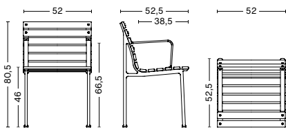
TRAVERSE ARMCHAIR Width 52 cm Depth 52,5 cm Height 80,5 cm Seat height 46 cm Seat depth 38,5 cm
