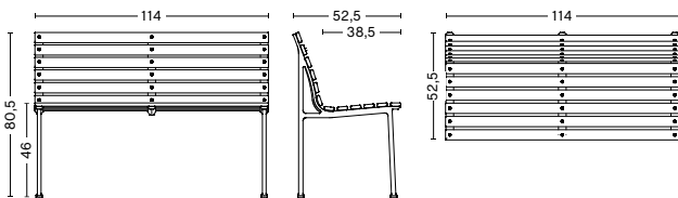
TRAVERSE DINING BENCH Width 114 cm Depth 52,5 cm Height 80,5 cm Seat height 46 cm Seat depth 38,5 cm
