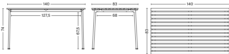
TRAVERSE TABLE Length 140 cm Width 83 cm Height 74 cm
