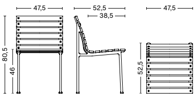
TRAVERSE CHAIR Width 47,5 cm Depth 52,5 cm Height 80,5 cm Seat height 46 cm Seat depth 38,5 cm
