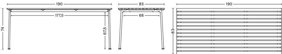
TRAVERSE TABLE Length 190 cm Width 83 cm Height 74 cm
