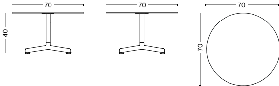
NEU TABLE LOW ROUND Diameter Ø70 cm Height 40 cm
