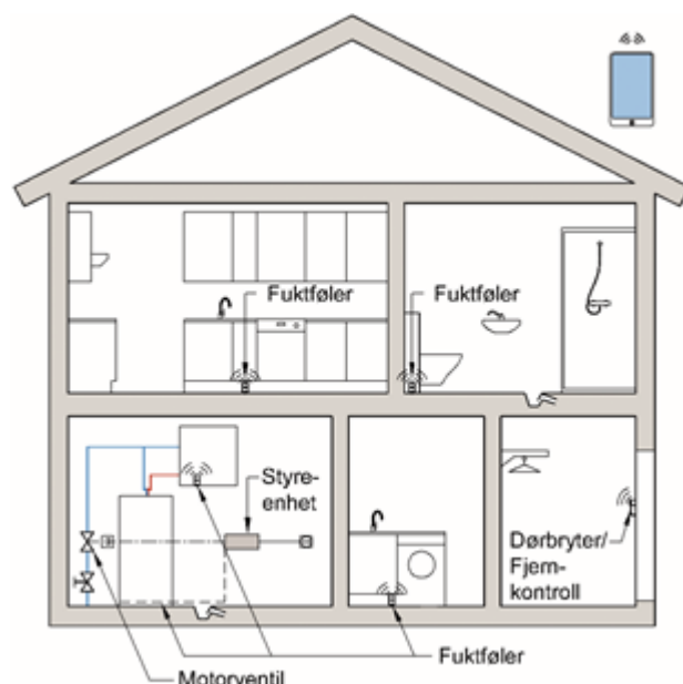
Fig. 1 Systemskisse for FlowStop smart lekkasjestopper
