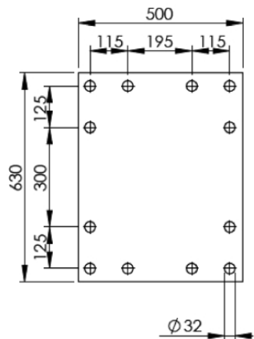
Gatenpatroon/hole pattern/ Bohrbild/motif de trous
