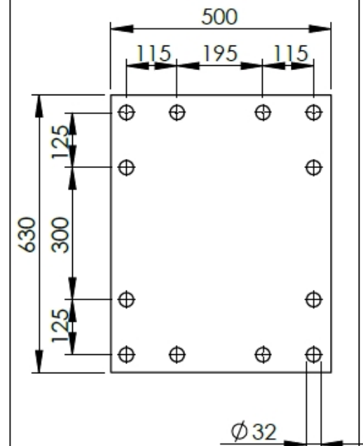
Gatenpatroon/hole pattern/ Bohrbild/motif de trous
