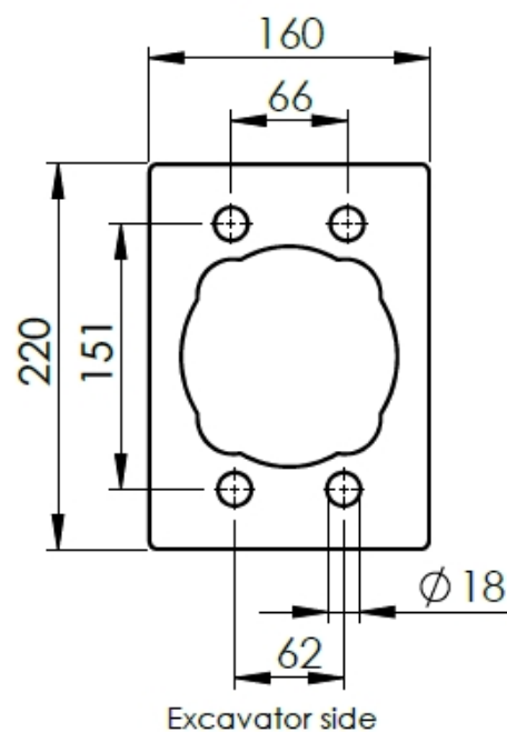
Gatenpatroon/hole pattern/ Bohrbild/motif de trous
