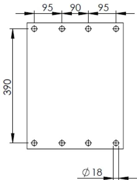
Gatenpatroon/hole pattern/ Bohrbild/motif de trous
