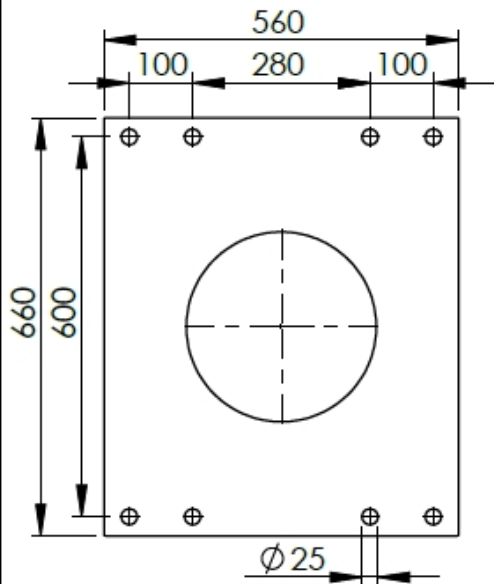
Gatenpatroon/hole pattern/ Bohrbild/motif de trous
