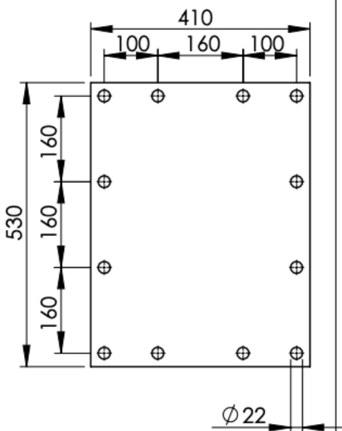
Gatenpatroon/hole pattern/ Bohrbild/motif de trous
