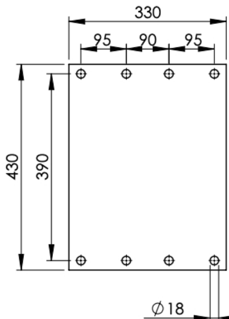
Gatenpatroon/hole pattern/ Bohrbild/motif de trous
