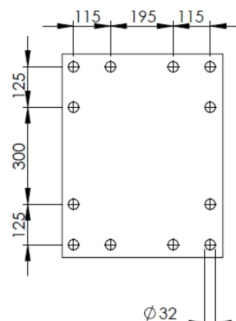
Gatenpatroon/hole pattern/ Bohrbild/motif de trous
