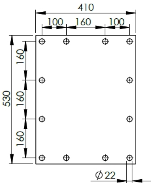
Gatenpatroon/hole pattern/ Bohrbild/motif de trous
