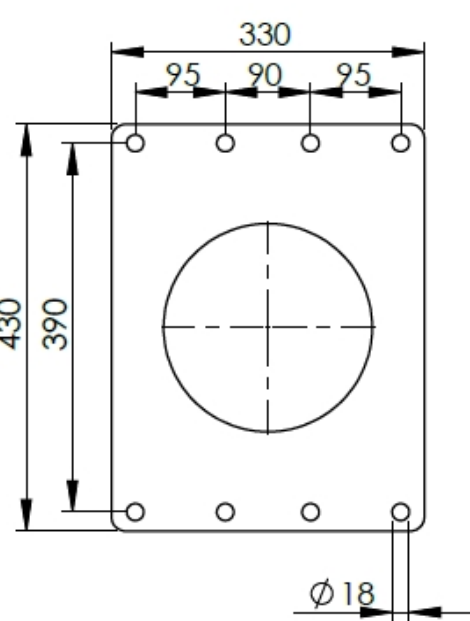
Gatenpatroon/hole pattern/ Bohrbild/motif de trous
