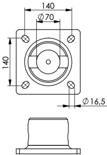
Gatenpatroon/hole pattern/ Bohrbild/motif de trous
