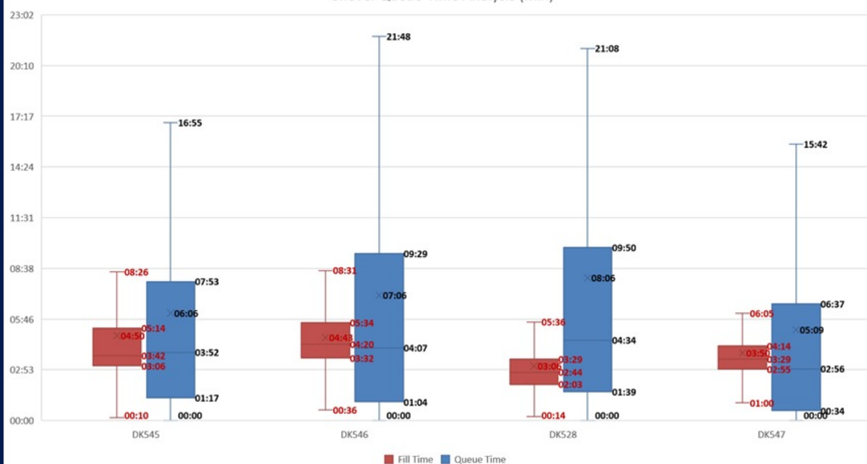
Shovel Queue Time Analysis (min)
