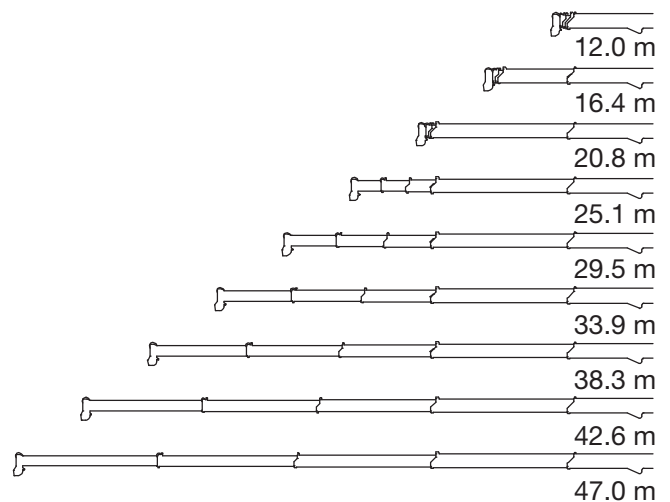
Boom Length
