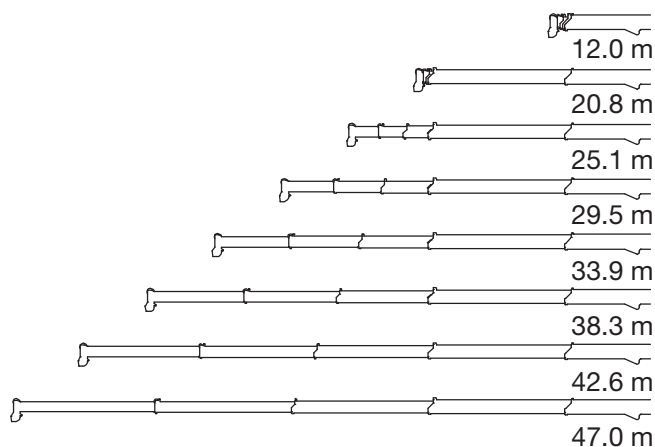
Boom Length
