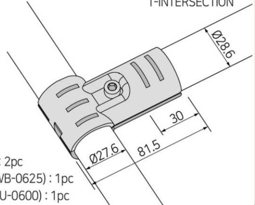
90 ° INTERCHANGEABLE JOINT (28mm/28.6mm) FOR CORNER OR T-INTERSECTION
