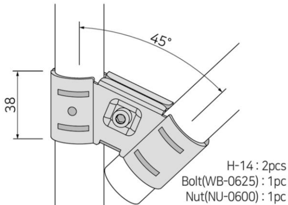
45 ° SUPPORT JOINT TO FORM AN ANGLE INTERSECTION
