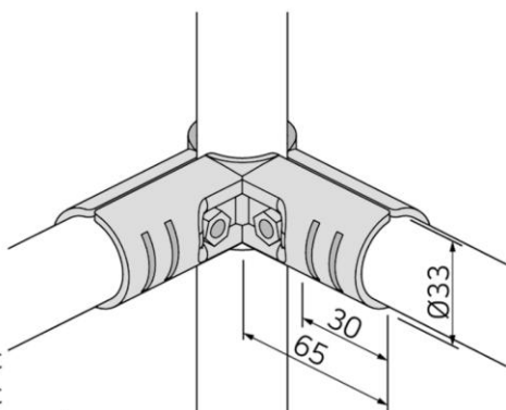
INSIDE CORNER JOINT TO FORM 3 WAY PIPE INTERSECTION
