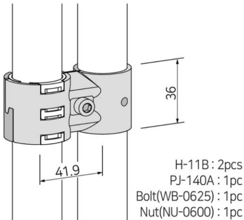
SINGLE HINGE JOINT TO CONNECT PARALLEL PIPE
