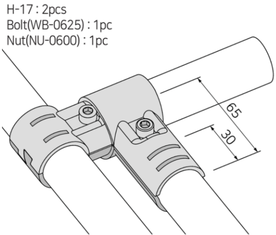
90 ° JOINT OVERSIZED
