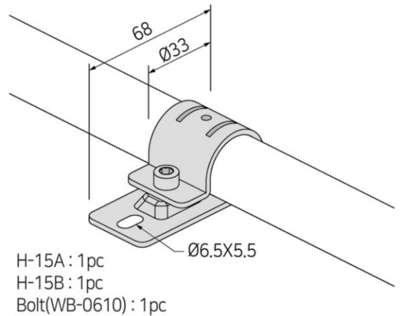
MOUNTING CLAMP
