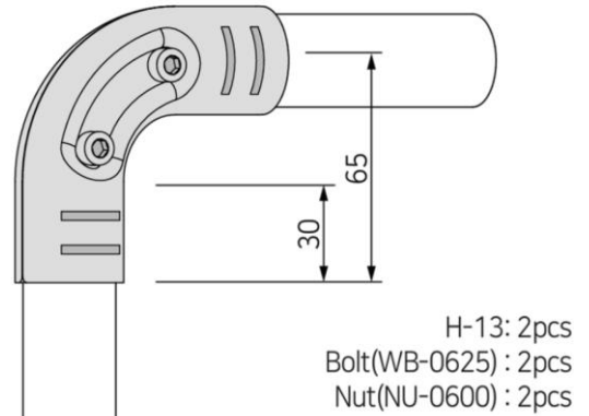
MOUNTING CLAMP
