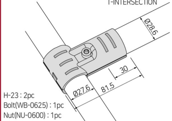
90 ° INTERCHANGEABLE JOINT (28mm/28.6mm) FOR CORNER OR T-INTERSECTION
