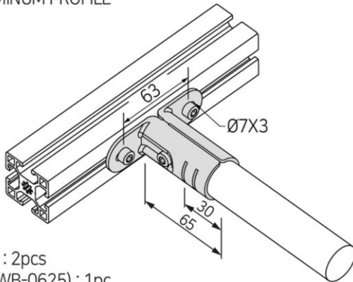
90 ° JOINT WITH FLAT END TO CONNECT ALUMINUM PROFILE
