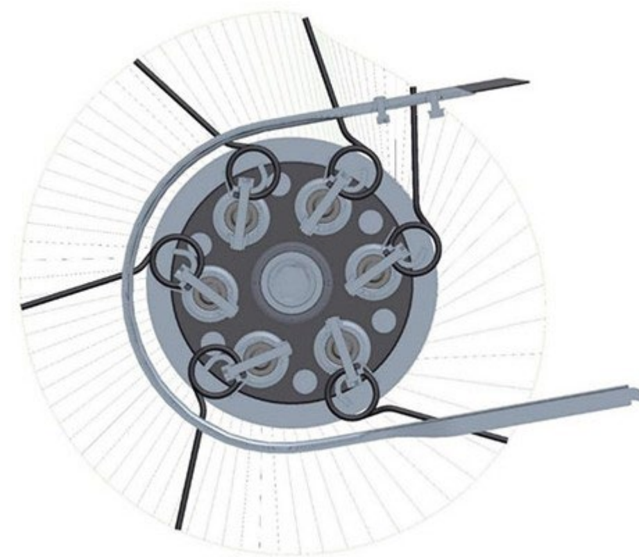
Six tine bar pickup reel
