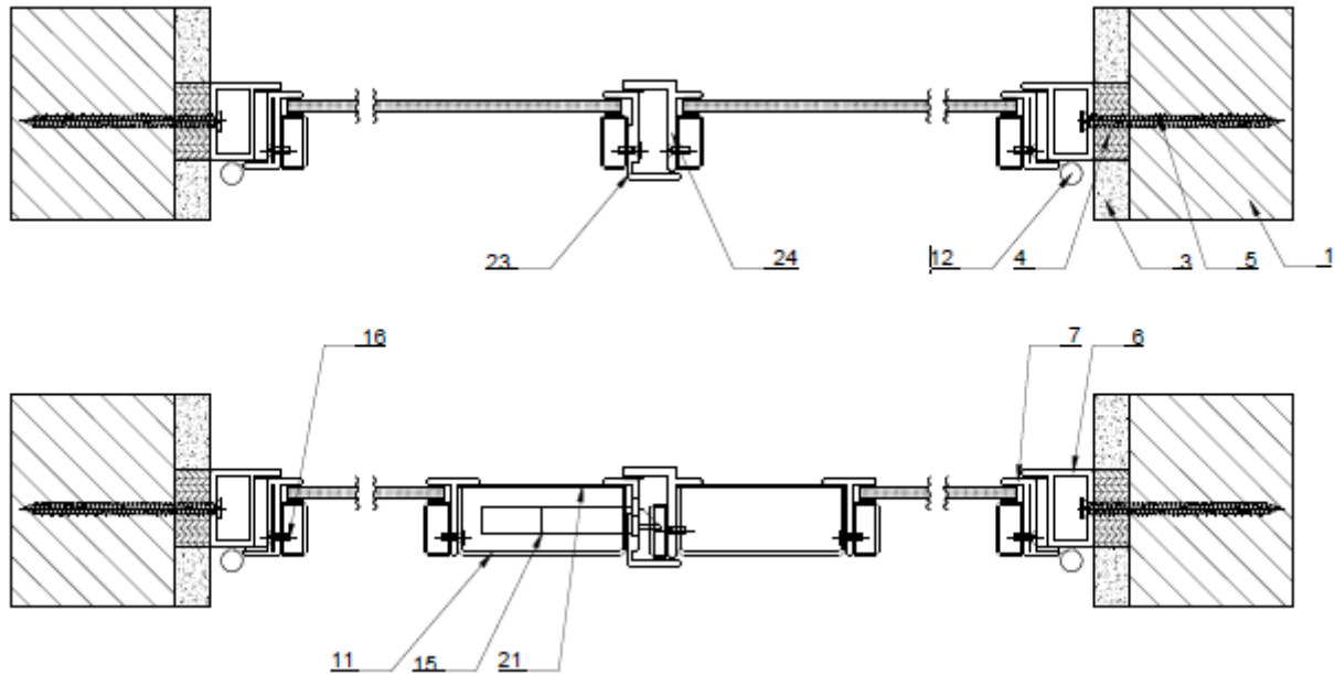
Fig. 3. Top projections of test elements. [Z]
