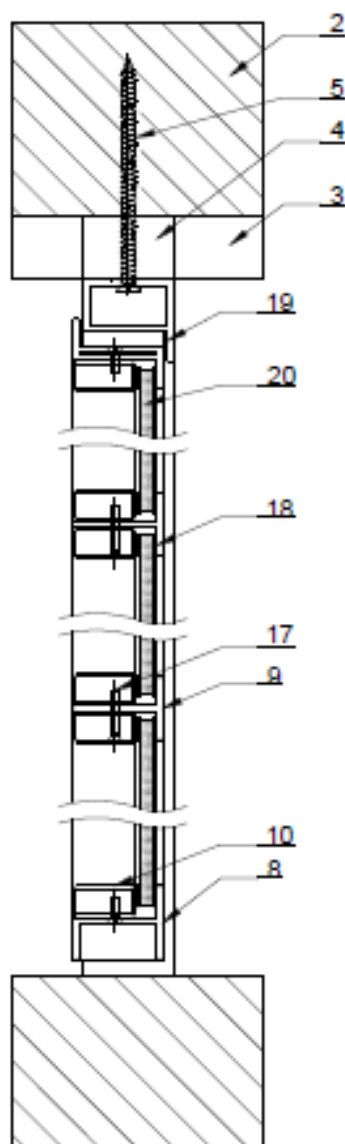
Fig.2. Side projections of test elements. [Z]
