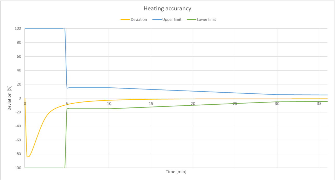
Chart 2. Heating accuracy chart.
