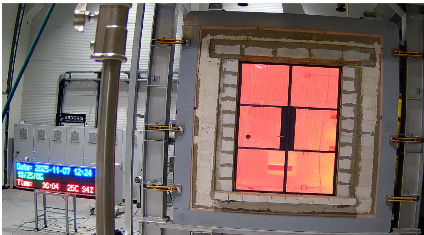
Photo. 2. Photo of the test piece after the test (36 min).
