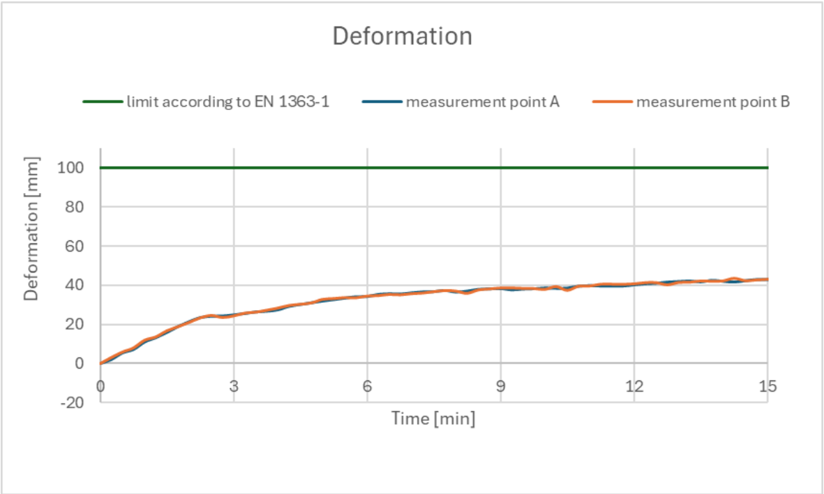
Chart 5. Deformation curve of the test piece
