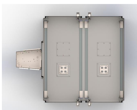
TOP CROSS SECTION VIEW OUTLET & COVER PLATE
