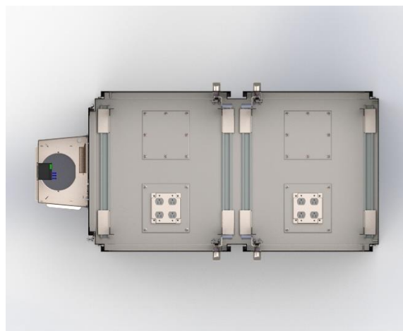
CROSS SECTION VIEW SHOWING QUAD BOXES AND ADAPTOR PLATES
