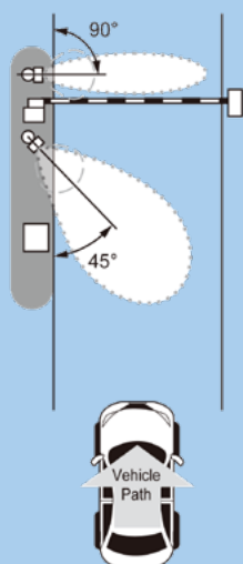
Barrier Gate
