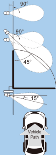
Swing Gate
