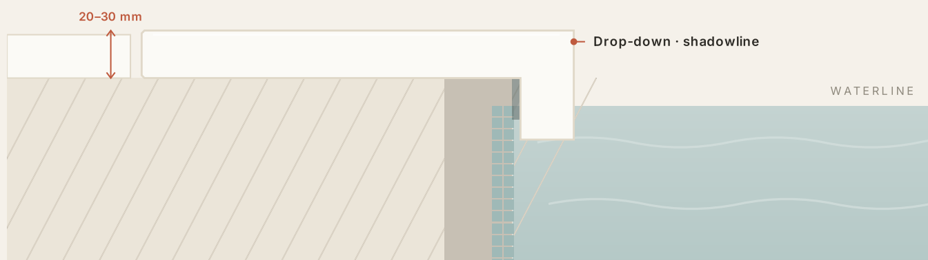
Section — solid-block coping returning over the beam to form the shadowline.
