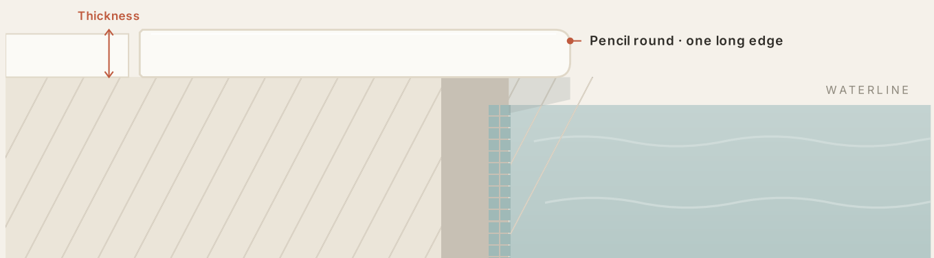
Section — top and bottom arris eased to a pencil round, flat face between.
