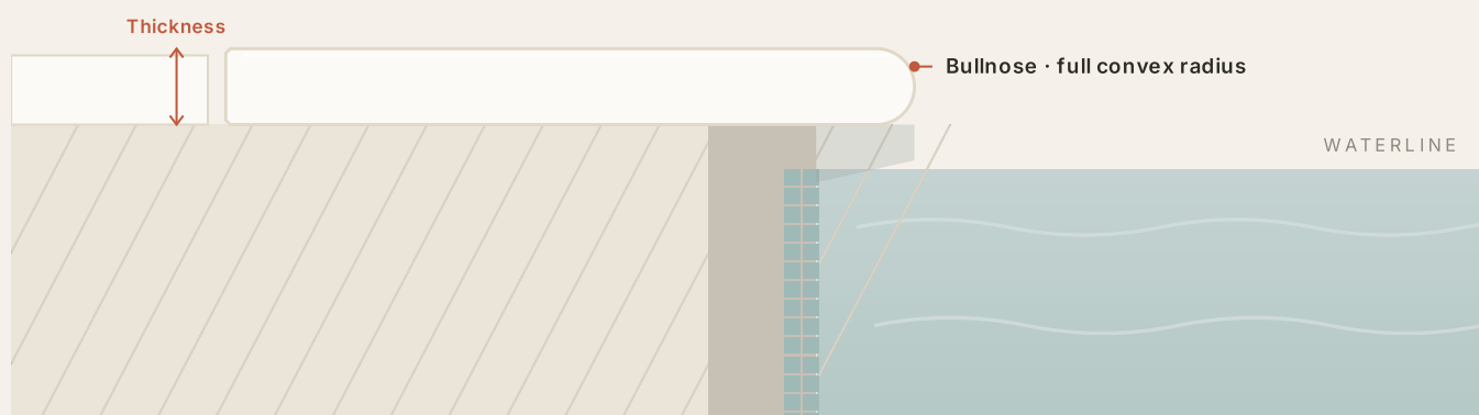
Section — a single convex radius across the full front edge.
