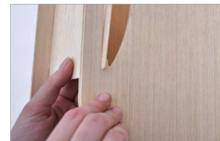
8. Verify that all corners of B are installed forward.
