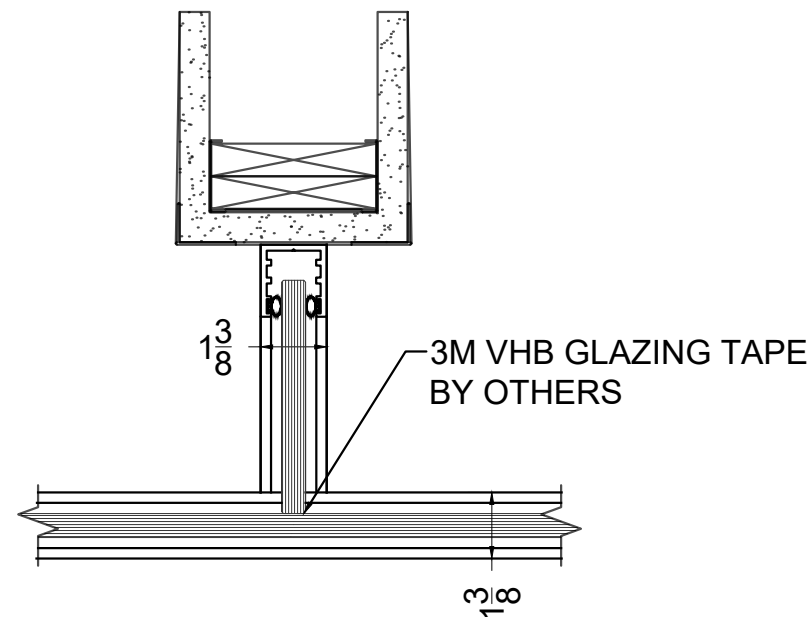
12 Z1 LH DOOR W / LADDER PULL - SINGLE GLAZE - WALL TO FIXED GLAZE 3" = 1' HORIZ. SECTION @ LH DOOR
