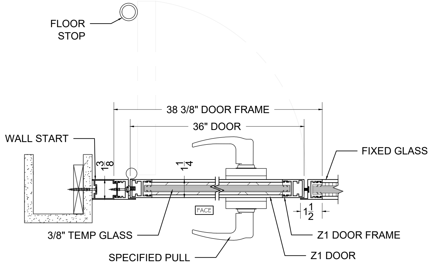
12 Z1 LH DOOR W / LADDER PULL - SINGLE GLAZE - WALL TO FIXED GLAZE 3" = 1' HORIZ. SECTION @ LH DOOR
