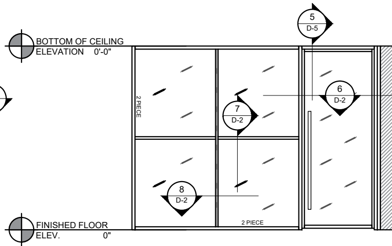
2 Z1 - VERTICAL & HORIZONTAL SASH EXAMPLE FREE SWING DOOR W/ LADDER PULL & STARTER
