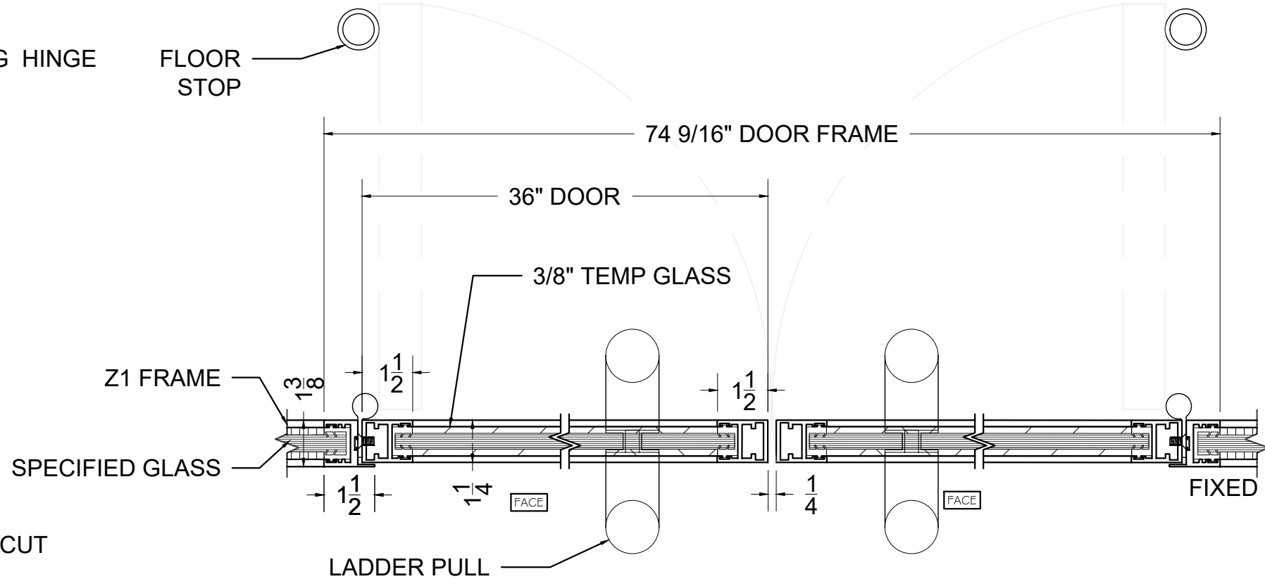
10 Z1 SINGLE GLAZE - POST FLY BY DIVIDER WALL 3" = 1' HORIZONTAL SECTION @ DIVIDER WALL
