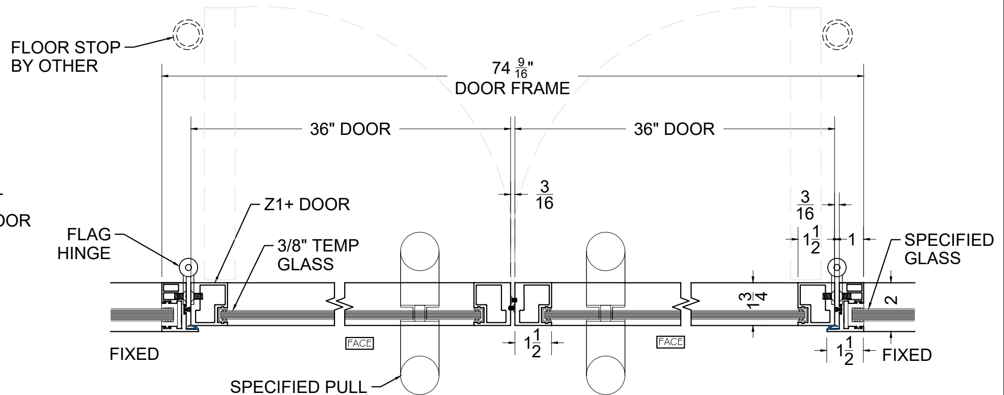
10 Z1+ POST FLY BY DIVIDER WALL 3" = 1' HORIZONTAL SECTION
