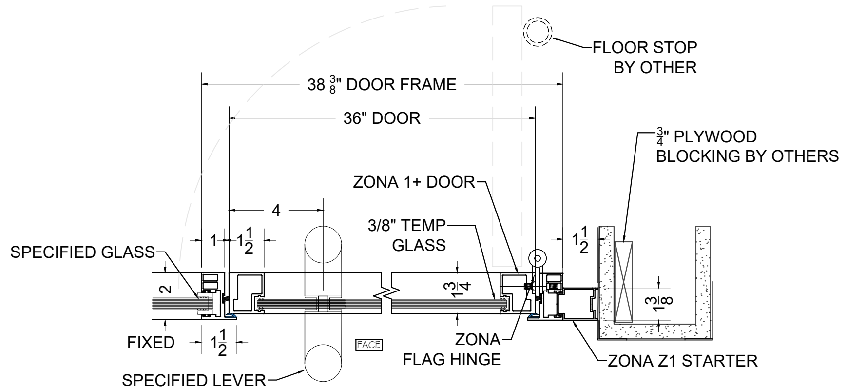
6 Z1+ RH DOOR W / LEVER PULL - DOOR @ PARTITION WALL 3" = 1'-0" HORIZ. SECTION
