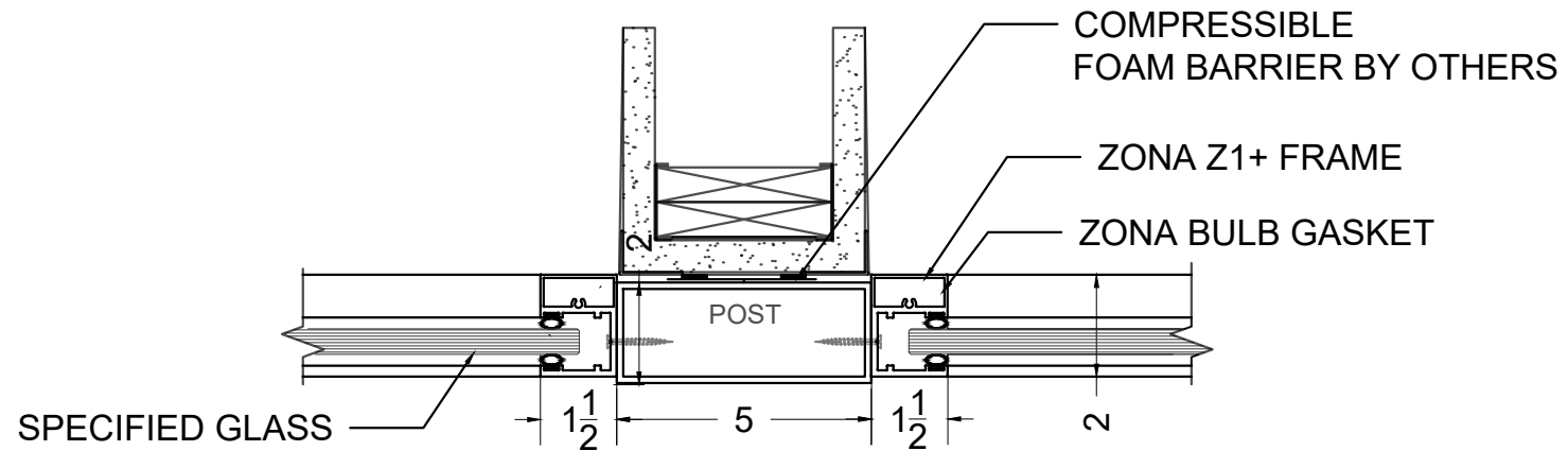
10 Z1+ POST FLY BY DIVIDER WALL 3" = 1' HORIZONTAL SECTION
