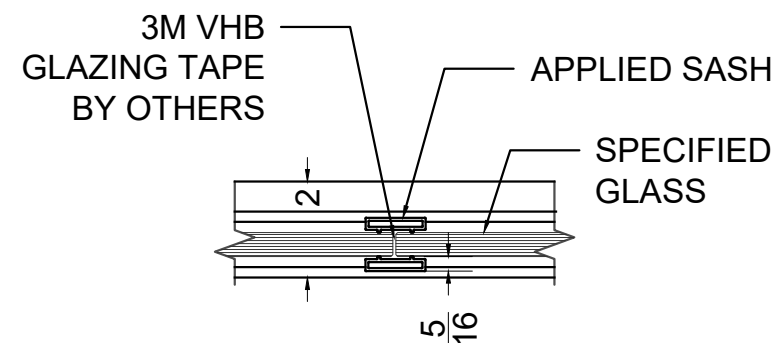
8 Z1+ SINGLE GLAZE - VERTICAL SASH 3" = 1' HORIZONTAL SECTION
