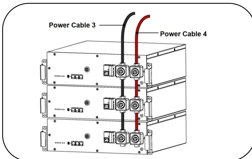
Figure 15 Sample of Connection for Inverter
