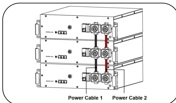
Figure 14 Sample of Power Connections Between Batteries
