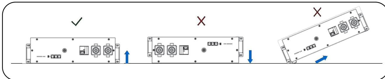
Figure 5 Installation Angle
