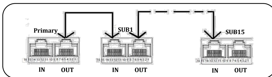
Figure 17 Sample of Communication Parallel
