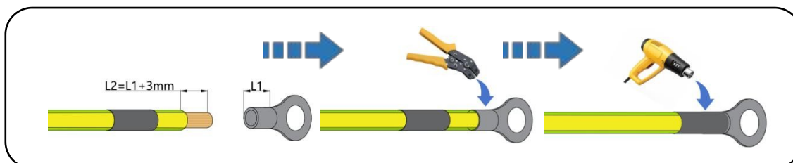
Figure 12 Sample of crimping method
