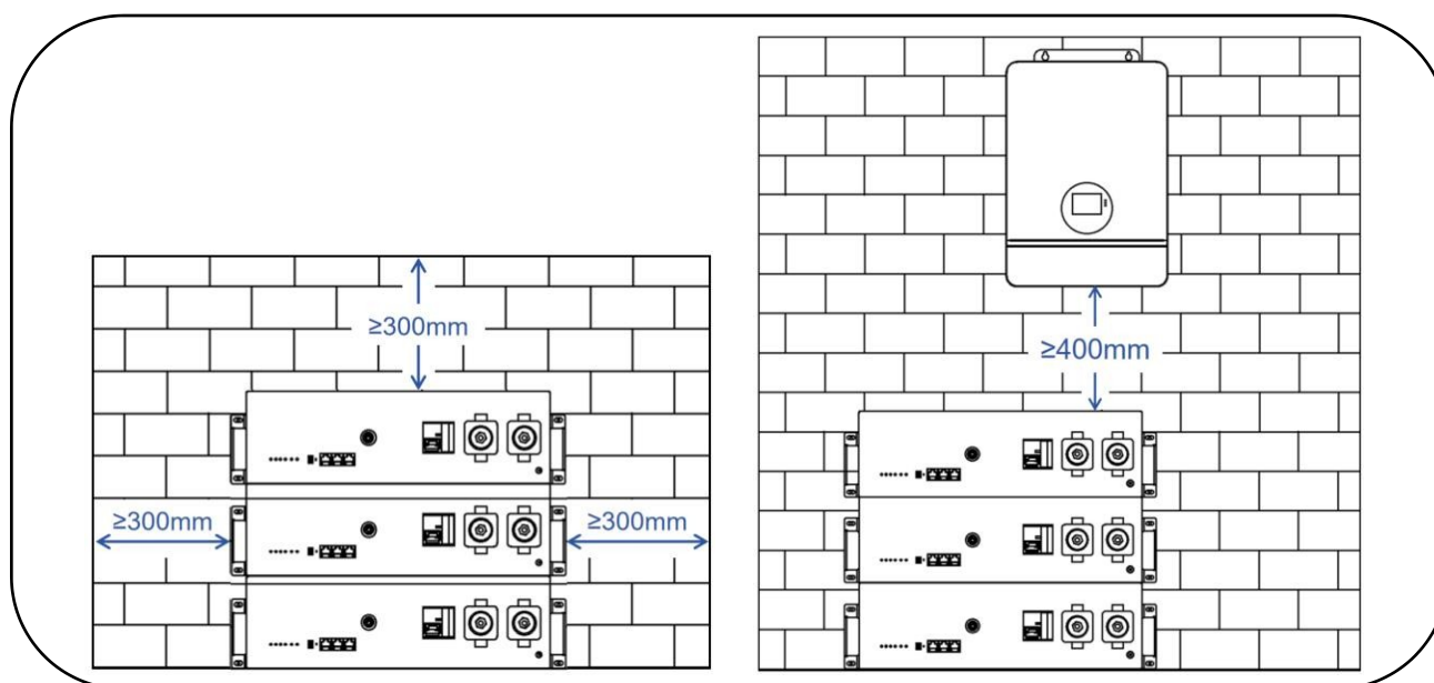
Figure 6 Installation Space
