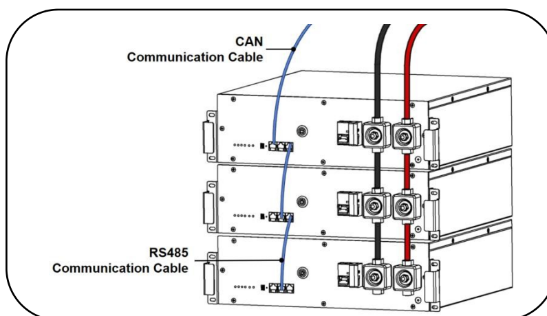
Figure 16 Sample of Connection for the Communication Cable
