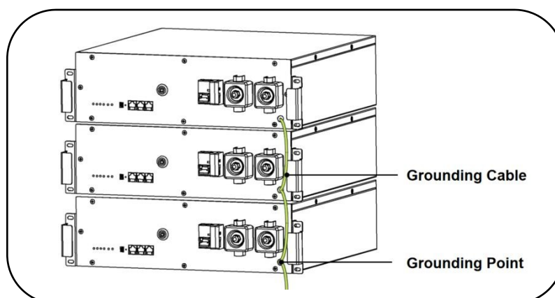
Figure 13 Sample of Battery Ground Connection
