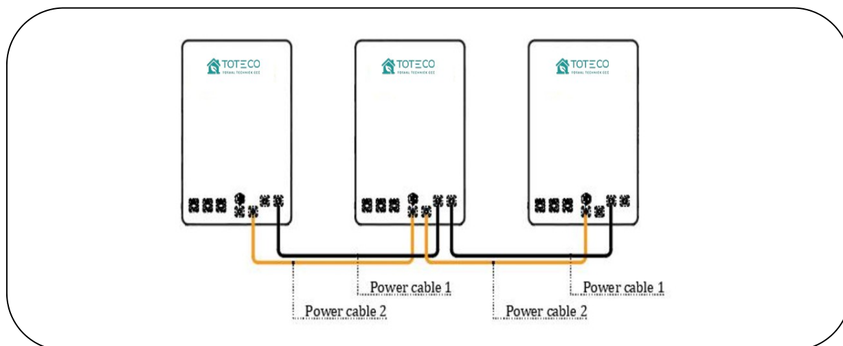
Figure 15 Sample of Power Connections Between Batteries
