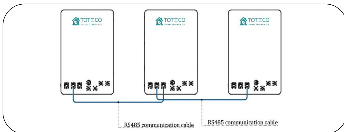
Figure 18 Sample of Connection the RS485 Communication Cable
