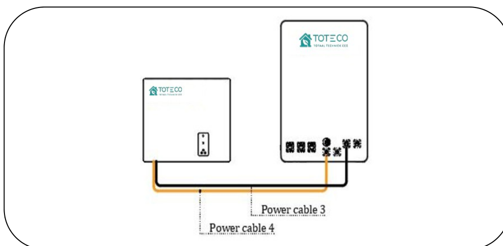
Figure 16 Sample of Power Cable Connection Between the Battery And Inverter
