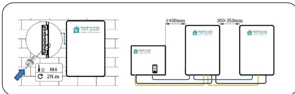
Figure 11 Sample of Step 3 For Wall Installation
