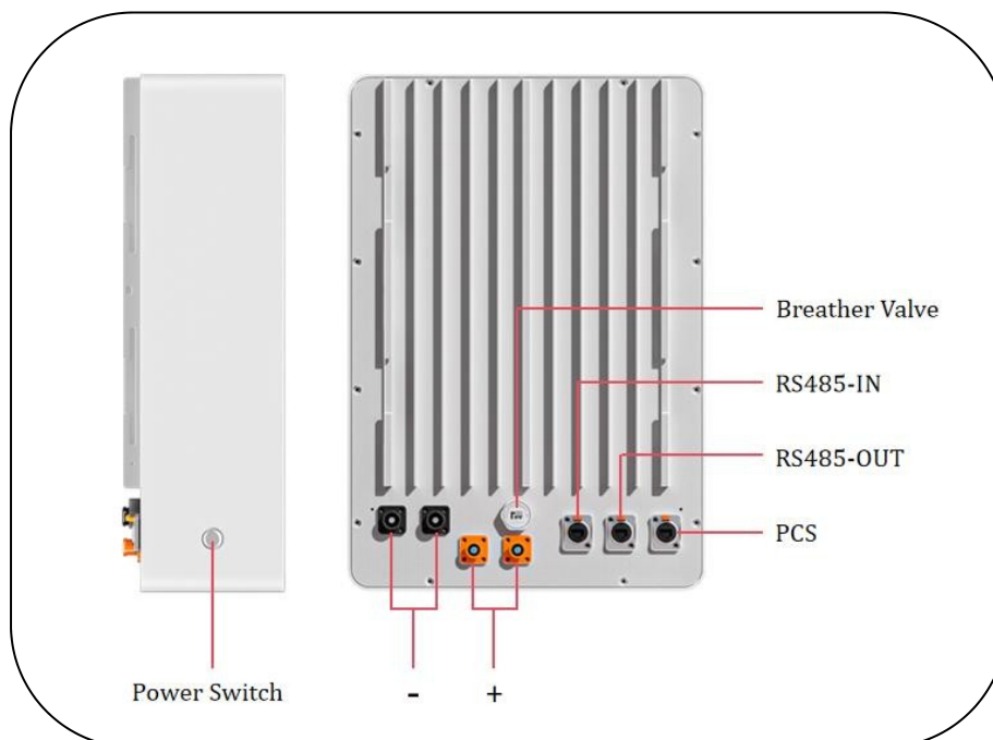
Figure 3 Interface Location Chart
