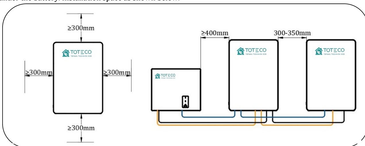
Figure 6 Installation Space
