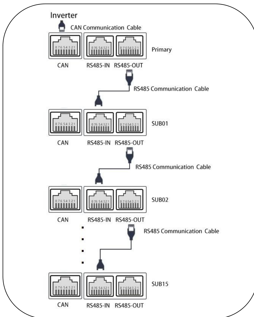
Figure 19 Sample of Communication Parallel
