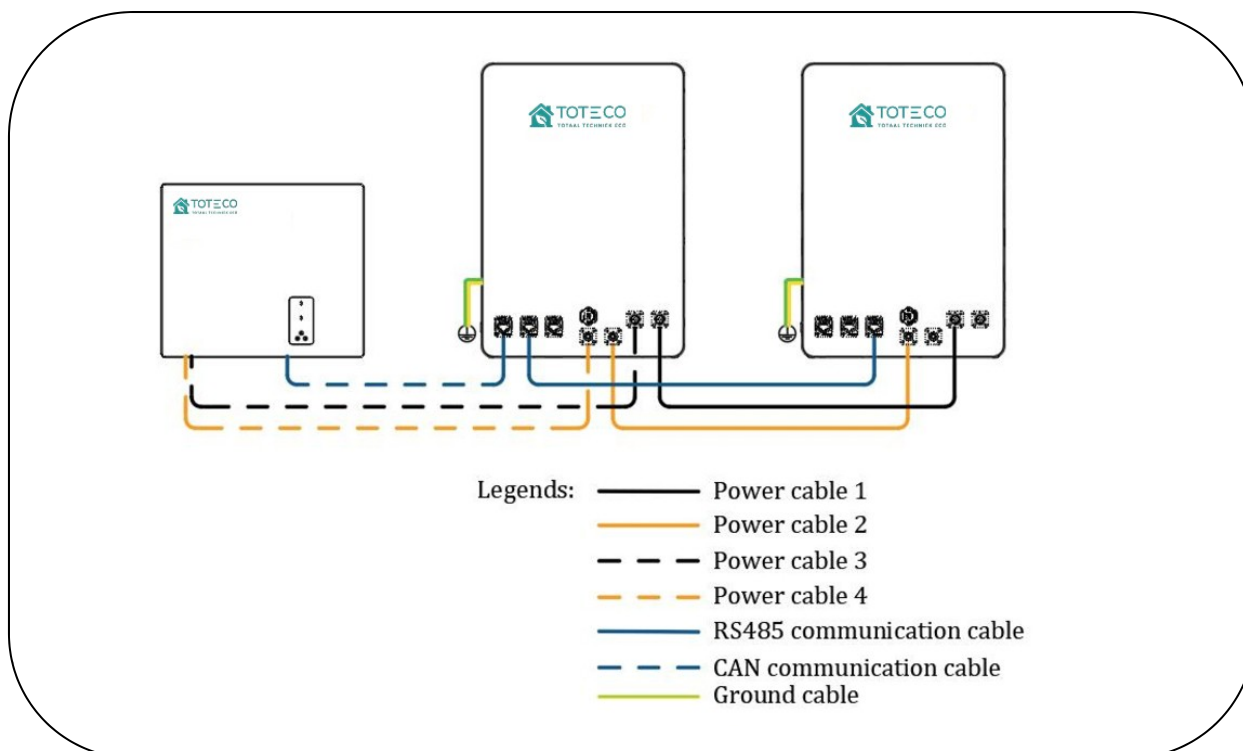
Figure 12 System General Wiring Diagram
