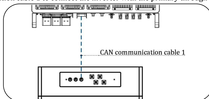
Figure 26 Sample of Connecting the CAN Communication Cable 1
