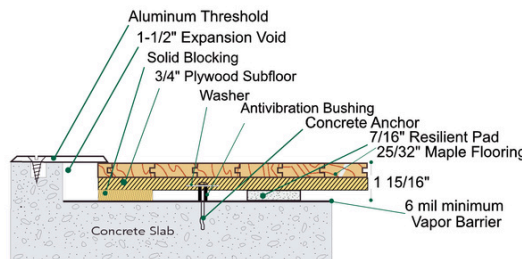
Threshold Detail (Optional Accessory)
