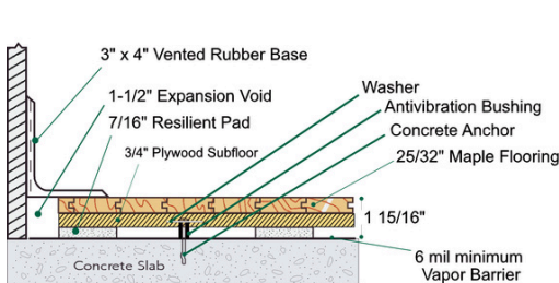
Wall Base Detail
