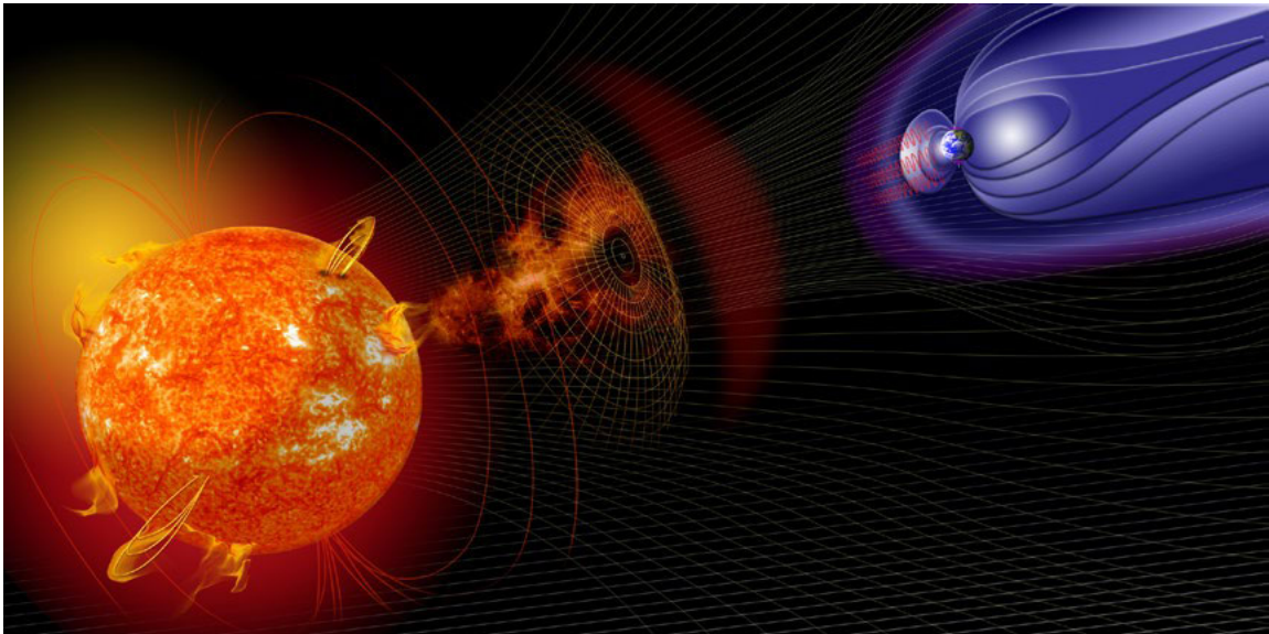
Figure 2: NASA rendering of stellar magnetic fields. In this image, the blue lines represent Earth's magnetic field that is distorted by the “solar wind.”
