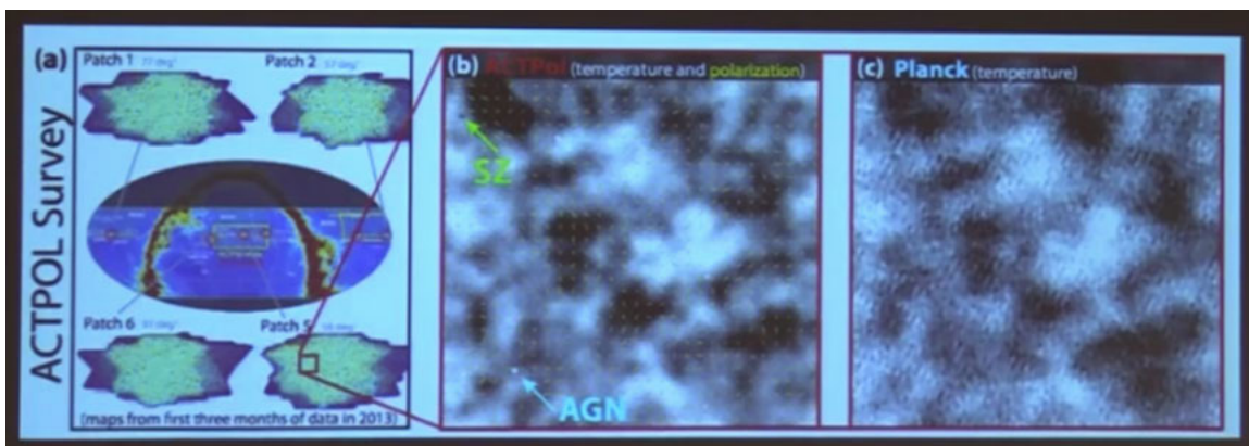
Figure 5: A slide from David Spergel's presentation: two greyscale pixel maps of the fluctuation pattern of the microwave background in a patch in the sky, one made with the Atacama Cosmology Telescope (center), the other with the Planck satellite (right). Source: https://www.youtube.com/watch?v=j3fHkQa6818 .
