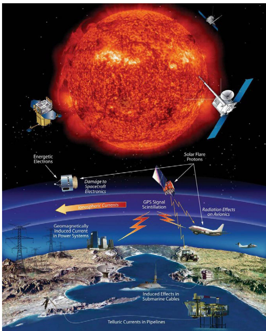
Figure 4: An image of the space-weathered world released by NASA. The caption that accompanies this image on NASA's website reads: "A web of inter-dependencies makes the modern economy especially sensitive to solar storms." Credit: https://www.nasa.gov .
