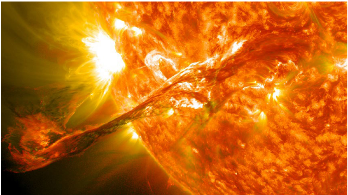
Figure 1: Extreme space weather events begin when plasma erupts from the Sun and streams towards Earth. This is an image of the Sun visualised in UV light by NASA’s Solar Dynamics Observatory (SDO). Credit: https://www.nasa.gov .
