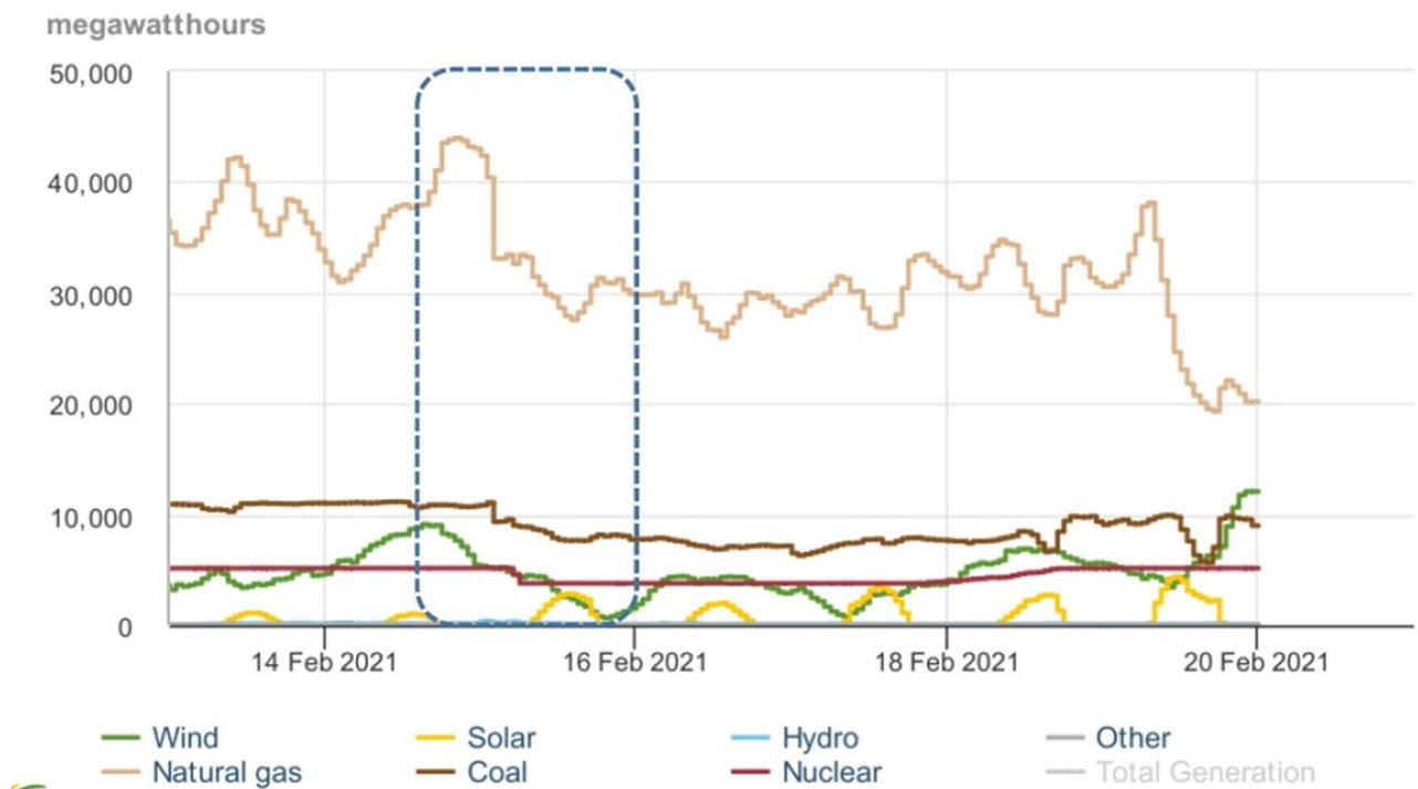
Figure 6: Generation mix, 14-20 February
