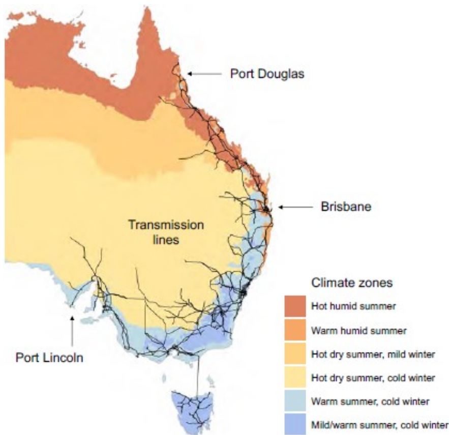
Figure 3: NEM weather zones
