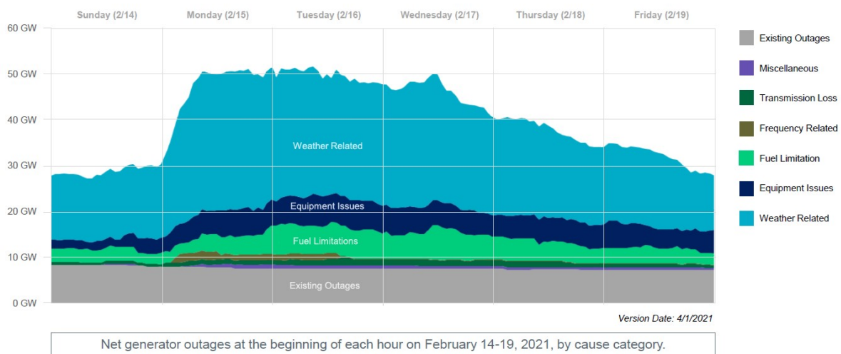
Figure 5: Generator outages by cause, 14-19 February
