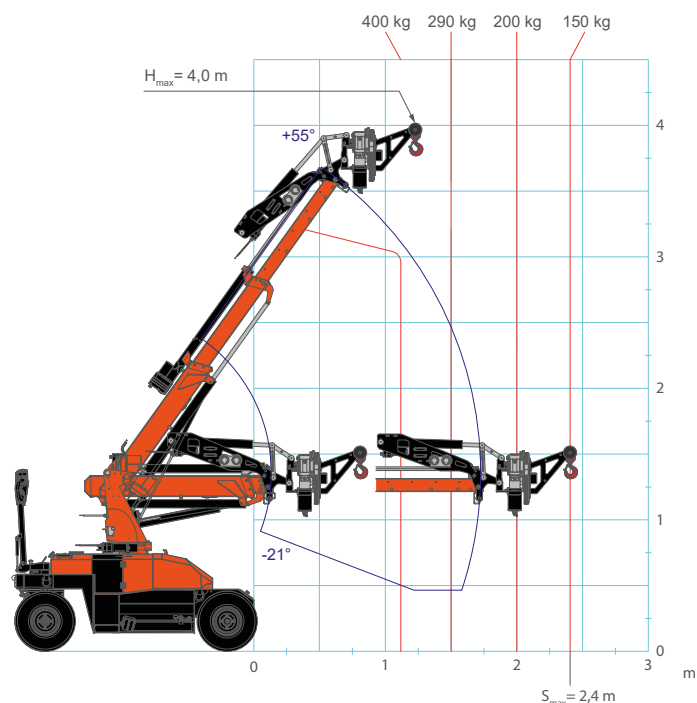
Manipulatorhaken-Lastdiagramm
