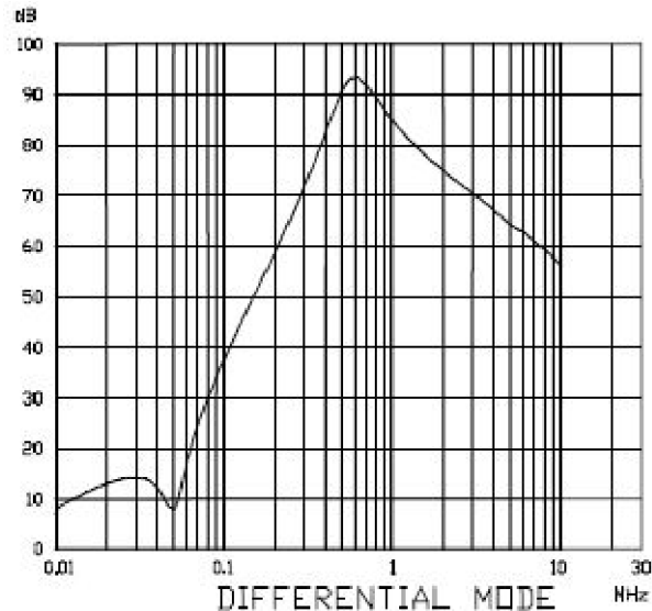
A2: 50/50Ω SYMMETRICAL (DIFFERENTIAL)
