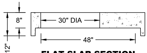
FLAT SLAB SECTION
