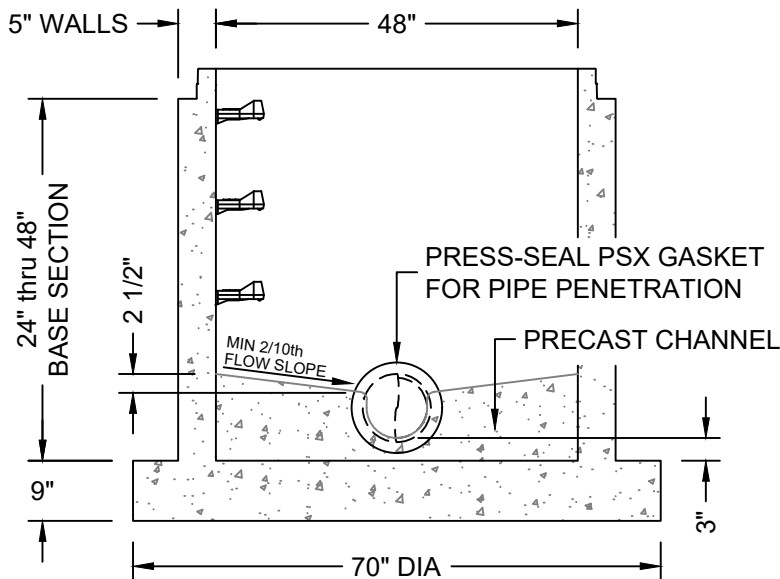
BASE SECTION
