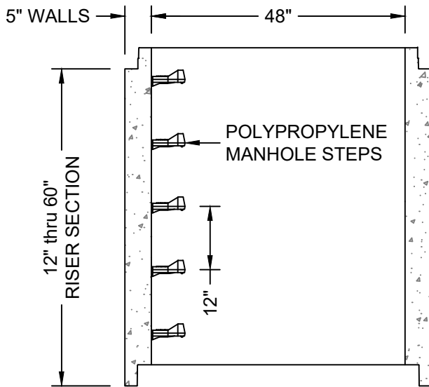
RISER SECTION
