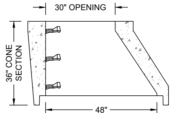
CONE SECTION
