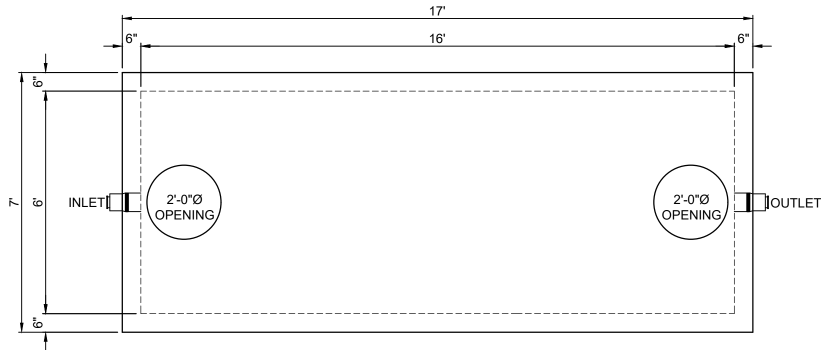
PLAN VIEW SCALE: 3/8" = 1'-0"
