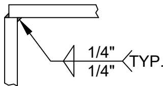
TYPICAL CORNER DETAIL
